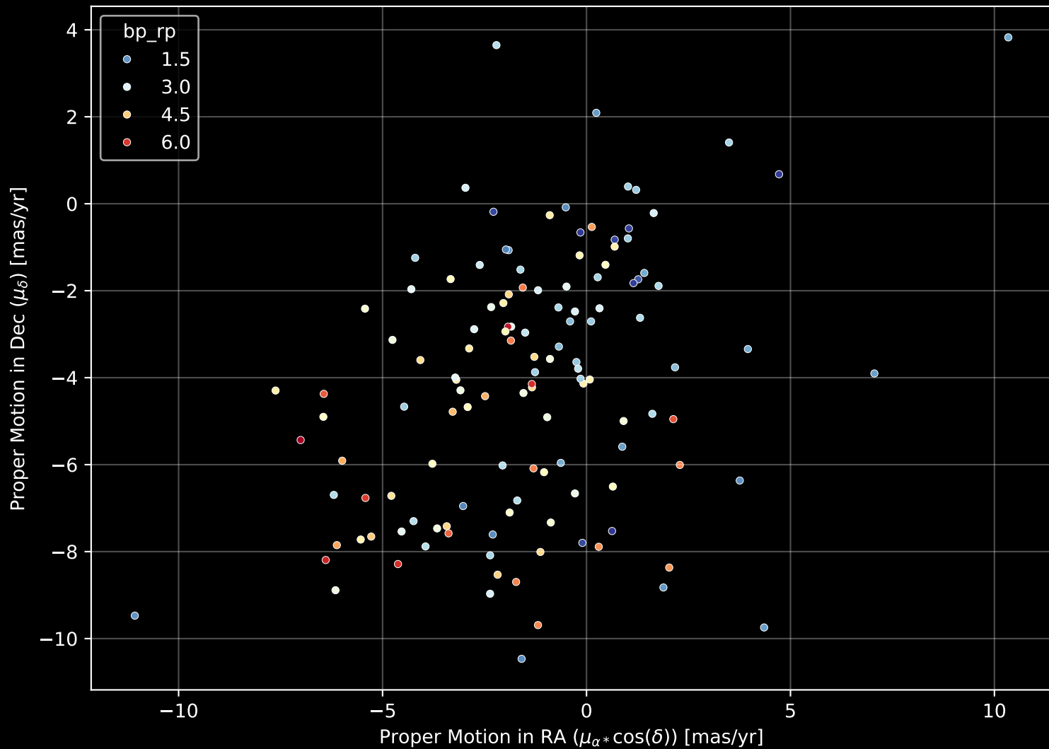
APOGEE DR17 Field: [008+02] Proper Motion Diagram (n= 129)
