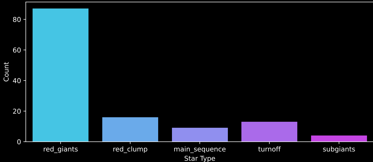
APOGEE DR17 Field: [008+02] Count plot of Star Type
