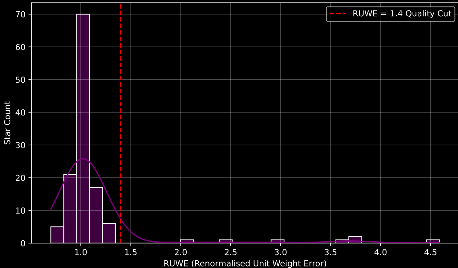
GAPOGEE DR17 Field [008+02] RUWE Distribution (n= 126)
