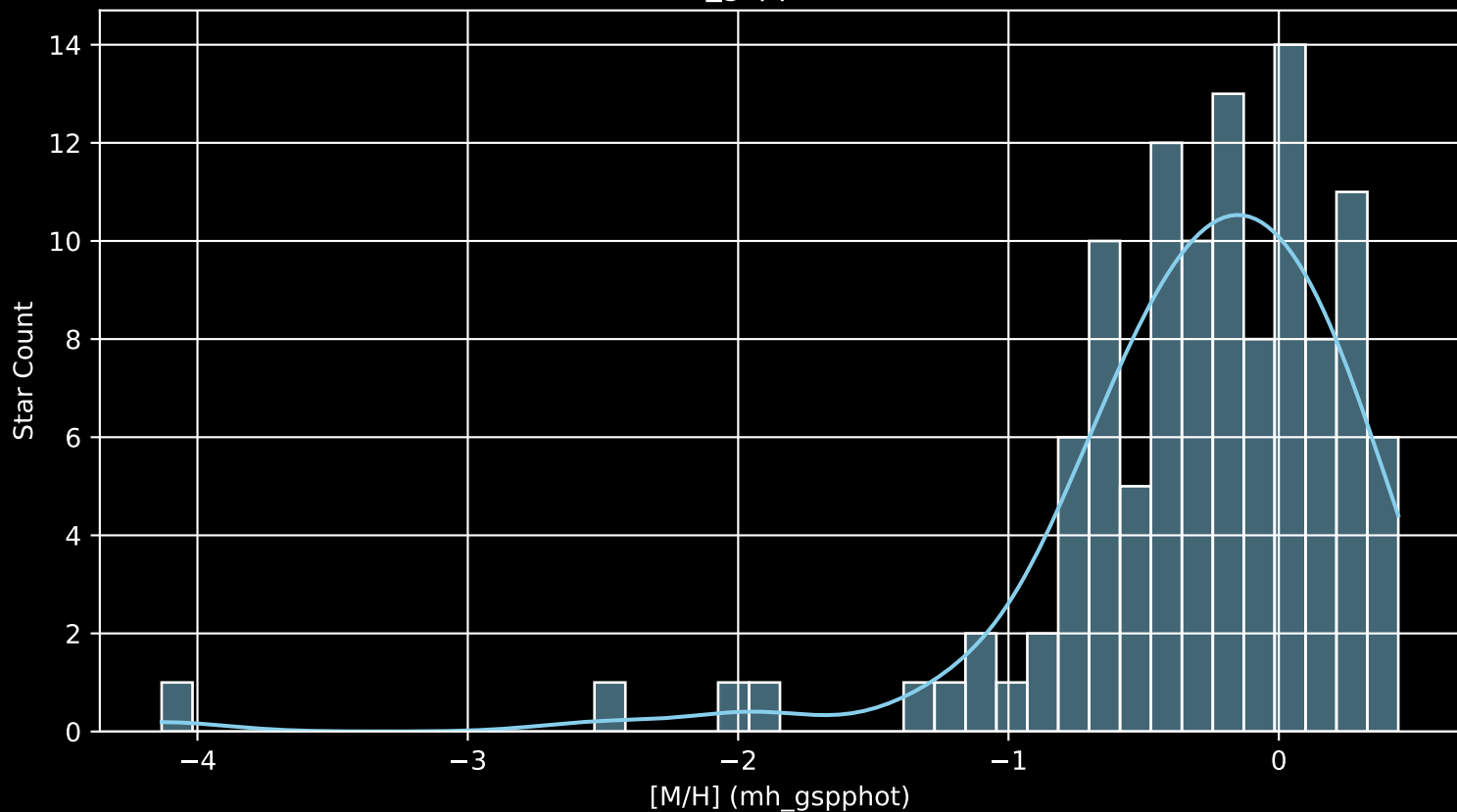
APOGEE DR17 Field: [008+02 [M/H] (mh_gspphot) (n= 114)
