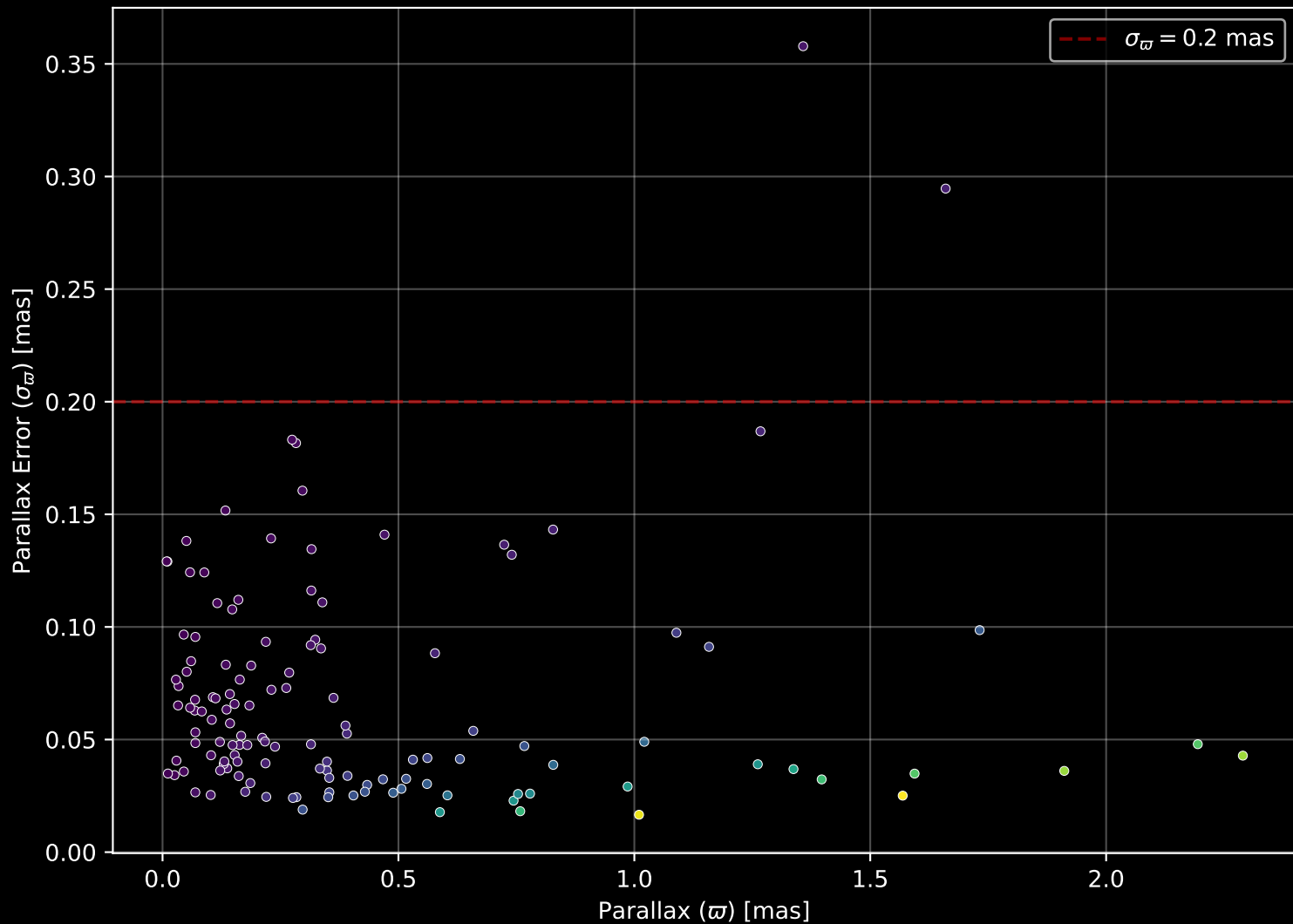
APOGEE DR17 Field: [008+02] Parallax Quality (n= 129)
