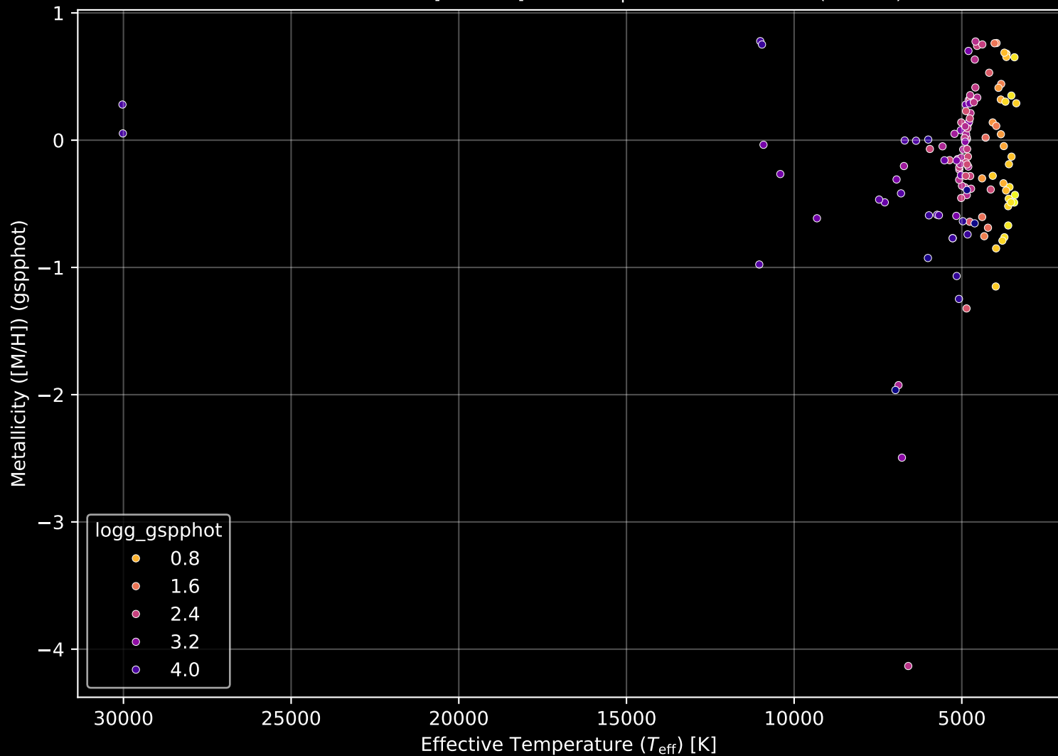
APOGEE DR17 Field: [008+02] Stellar Population Parameters (n= 129)
